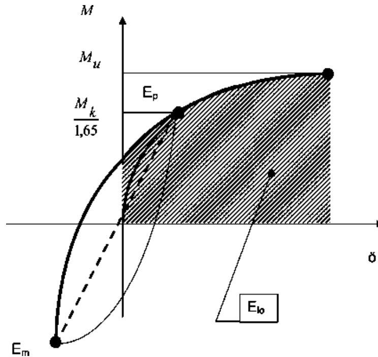
Figure 2 — Example for the determination of E_{i0} in case of a variant of the hysteresis loop
